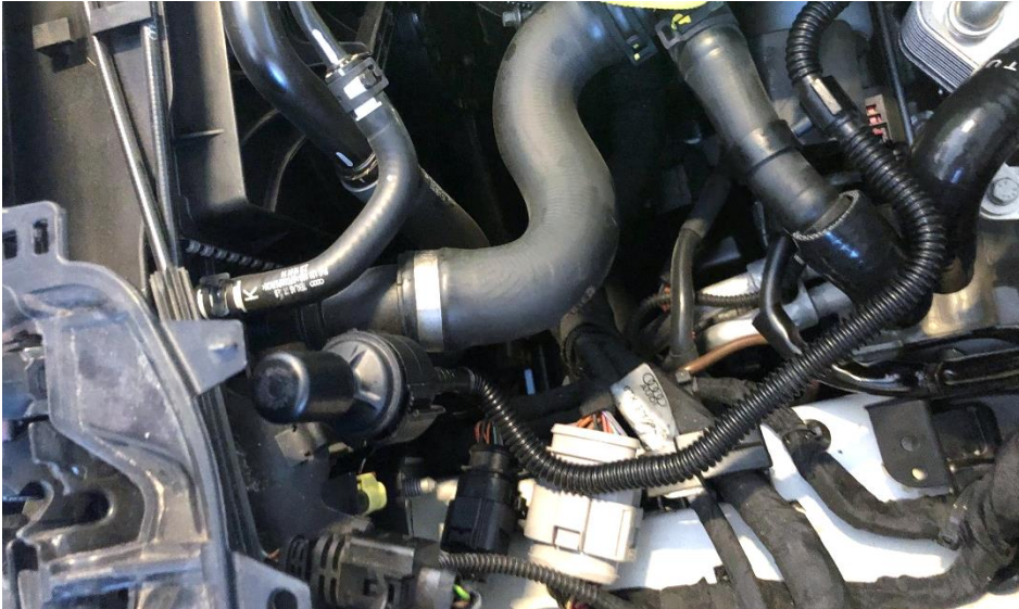
29. Route the Oil breather pot to the panel behind the headlamp – make sure the oil line is routed as shown
