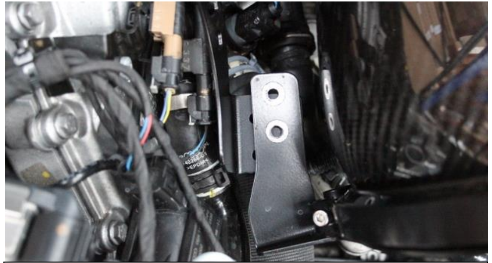
42. The bracket on the filter housing should be flat against the previously mounted bracket. Do not align then yet. Push the housing back as far as possible. We need clearance for the duct.
