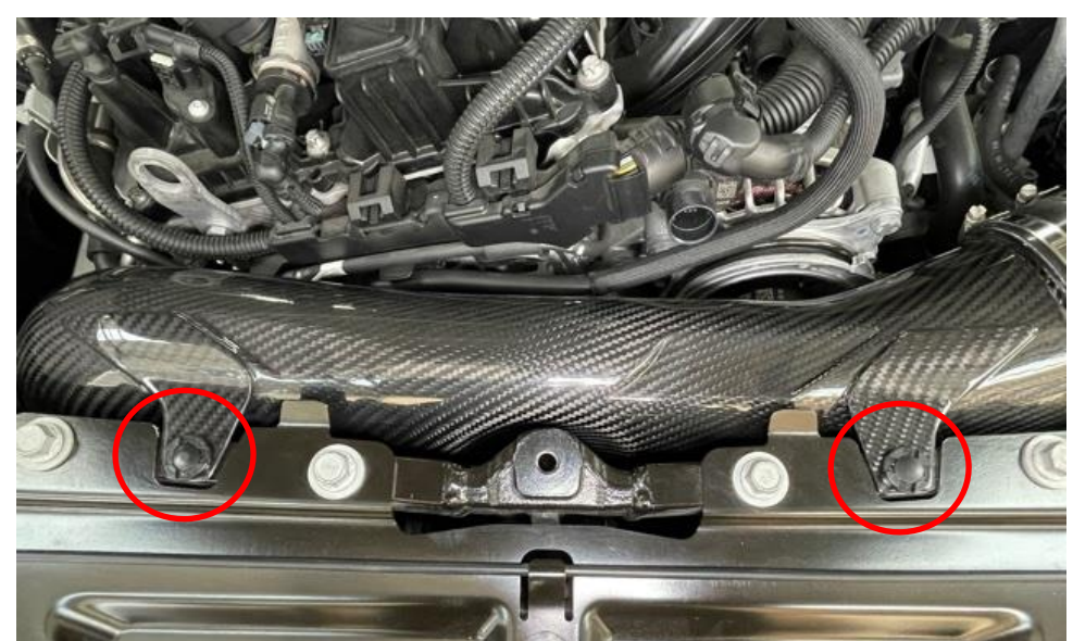
39. Use the 2 supplied plastic push clips and secure the tube.
