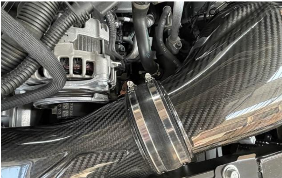
42. Tighten the hose clamps around the tube and housing - do not overtighten otherwise you can damage the carbon.
