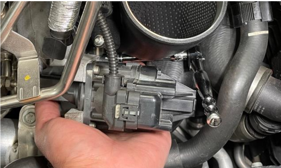
22. Once the screw has caught the thread - use a ratchet to tighten - again you can support the extension as shown.
